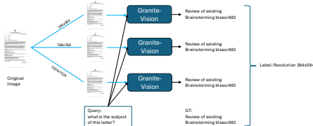
Figure 6: Label generation pipeline for training CARES. For each image-query pair, we evaluate a pre-trained VLM at multiple fixed resolutions and assign the smallest resolution that satisfies the sufficiency criterion as the supervision label.
