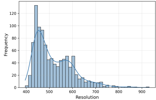
Figure 4: Histogram of the predicted resolutions \tilde{r} by CARES for OCRBench.
